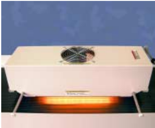
Shown here is the TB-499 drying unit. The extra wide heating area maximizes the effectiveness of the 2,300 BTU heater.
